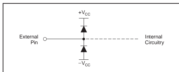
Figure 86. Internal ESD Protection
