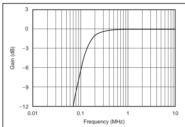
Figure 82. Frequency Response for the Filter of Figure 81
