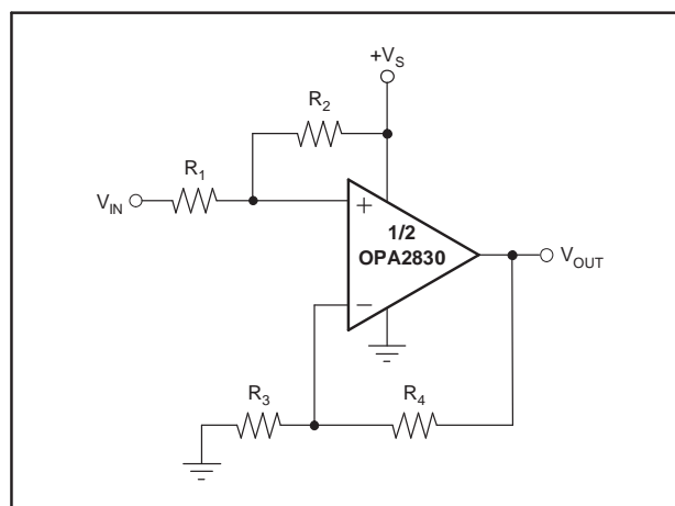
Figure 74. DC Level-Shifting
