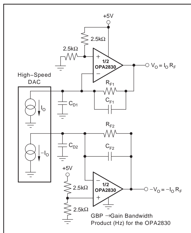
Figure 83. High-Speed DAC—Differential Transimpedance Amplifier
