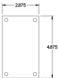
INNER PANEL
