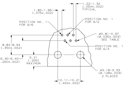
SUGGESTED PRINTED CIRCUIT BOARD MOUNTING HOLE LAYOUT VIEW SHOWN AS COMPONENT SIDE OF BOARD
