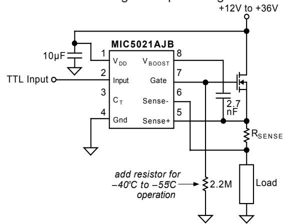
Figure 12b. Gate-to-Ground Pull Down
