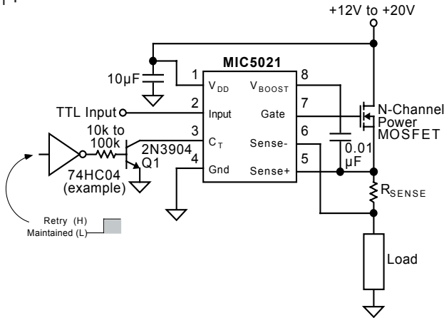
Figure 11. Remote Control Circuit
