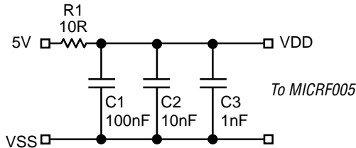
Figure 8. Supply Bypassing
