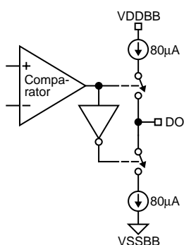
Figure 4. DO Pin
