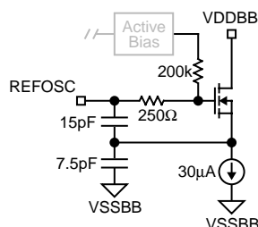
Figure 5. REFOSC Pin
