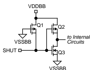
Figure 6. SHUT Pin
