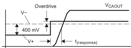
Figure 17. Overdrive Definition
