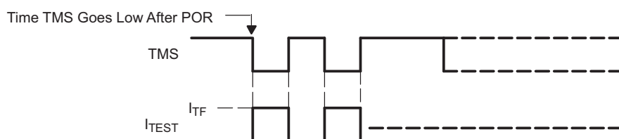
Figure 22. Fuse Check Mode Current
