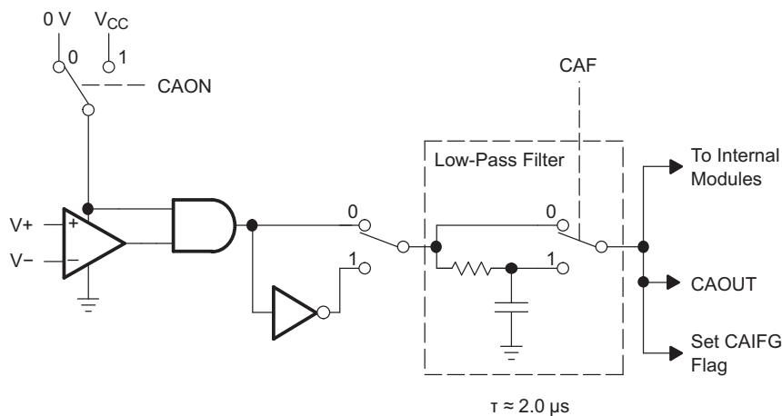
Figure 16. Comparator_A+ Module Block Diagram
