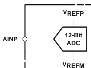
Figure 17. Single-Ended Input Stage
