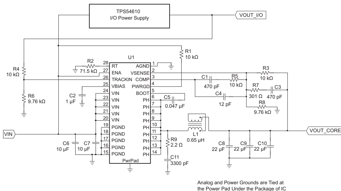
Figure 10. Application Circuit
