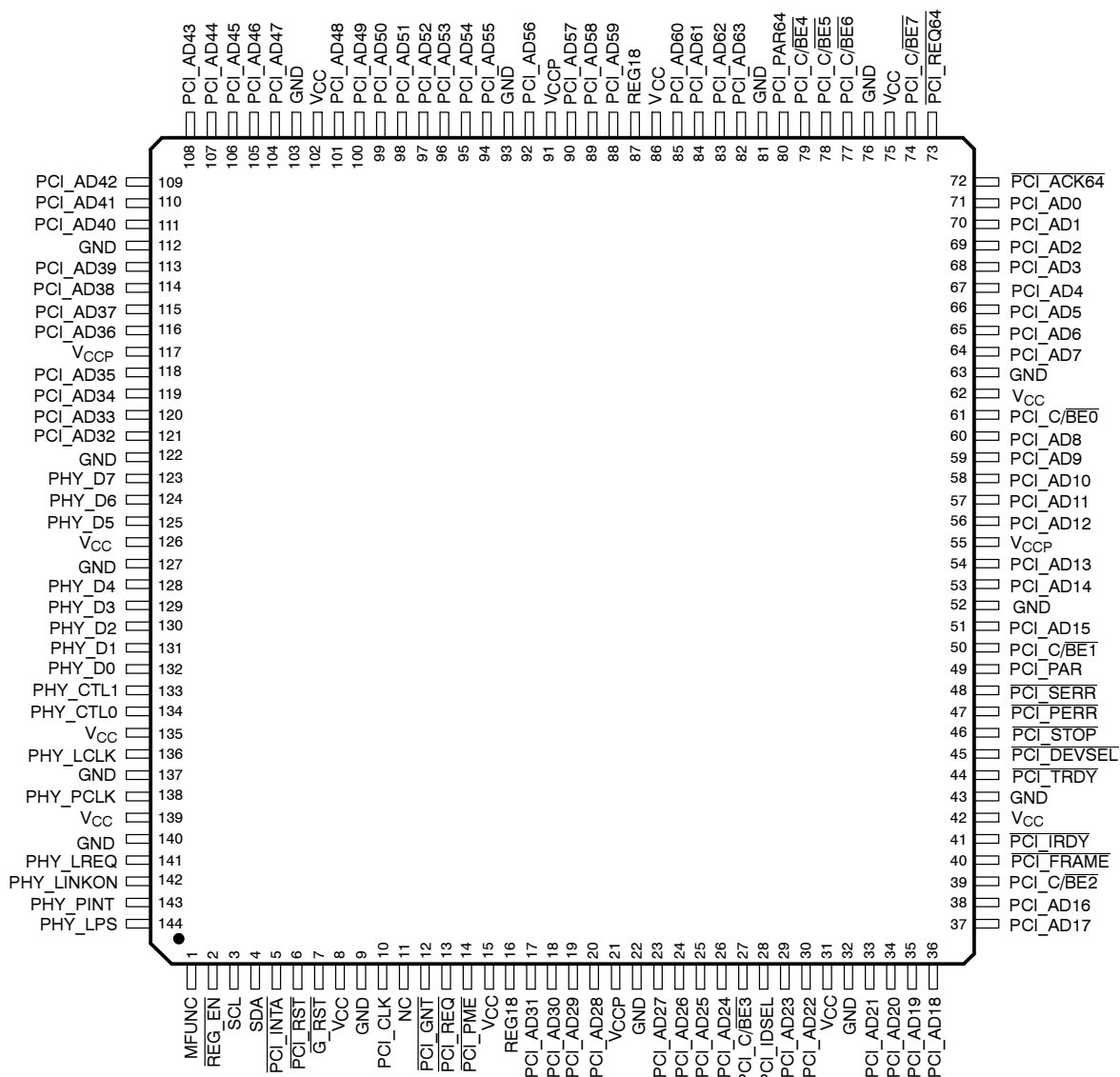
Figure 2-1. Terminal Assignments
