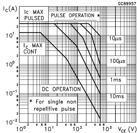
Figure 4: Derating Curve
