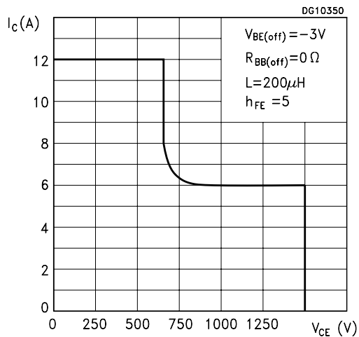
Figure 11: Reverse Biased Safe Operating Area
