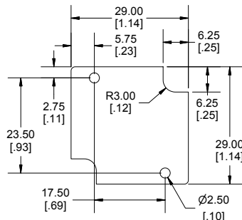
MAXIMUM P.C. BOARD SIZE
