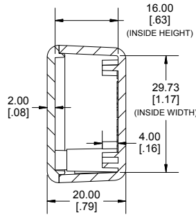
END VIEW SECTION B-B
