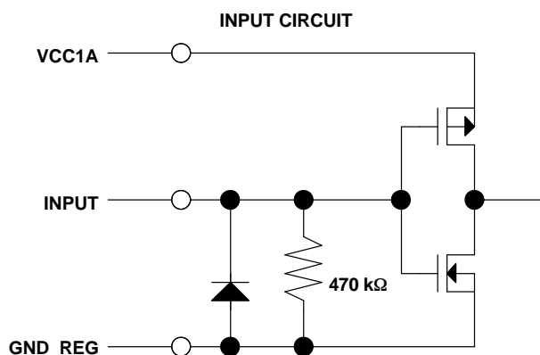
Figure 2. TLD
