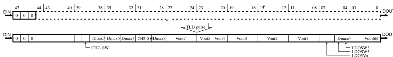
Figure 35. Shift Register Configuration and Changes for Test 0
