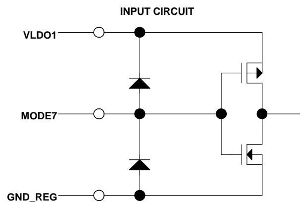
Figure 4. MODE7
