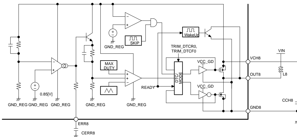
Figure 25. CH-8 Block Diagram
