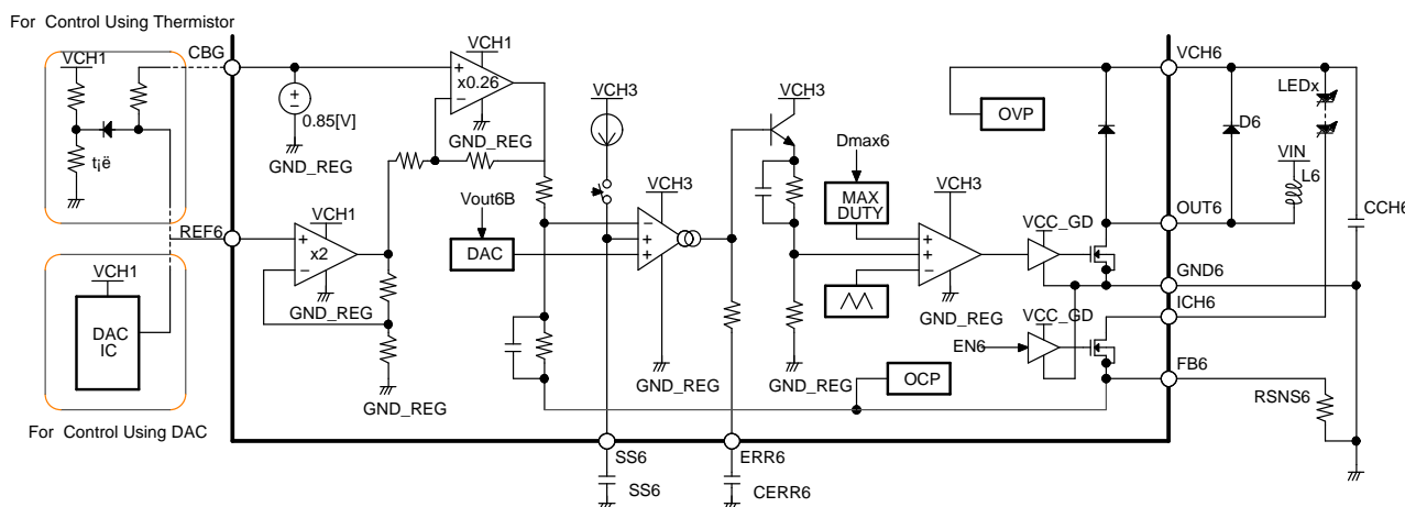
Figure 22. CH-6 Block Diagram
