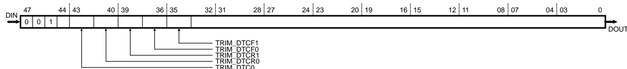
Figure 40. Shift Register Configuration for Test 1
