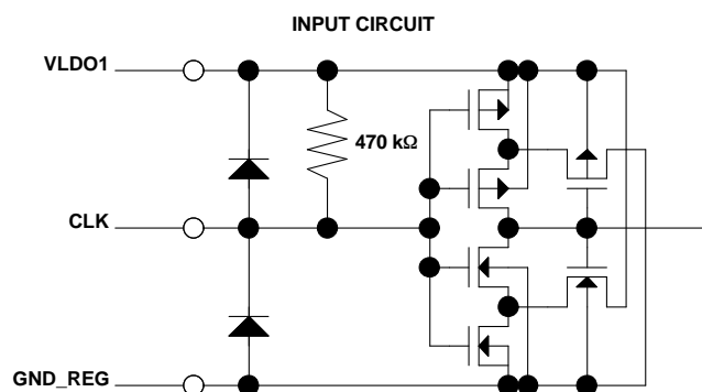
Figure 5. CLK
