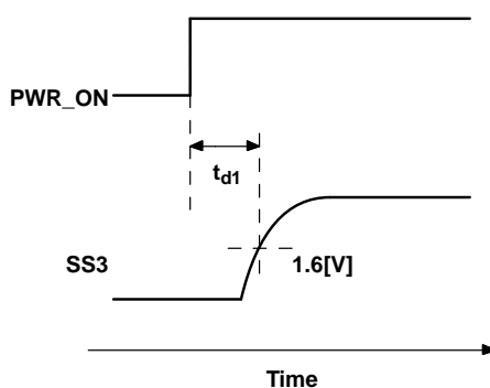
Figure 8. t_{d1} Measurement Reference
