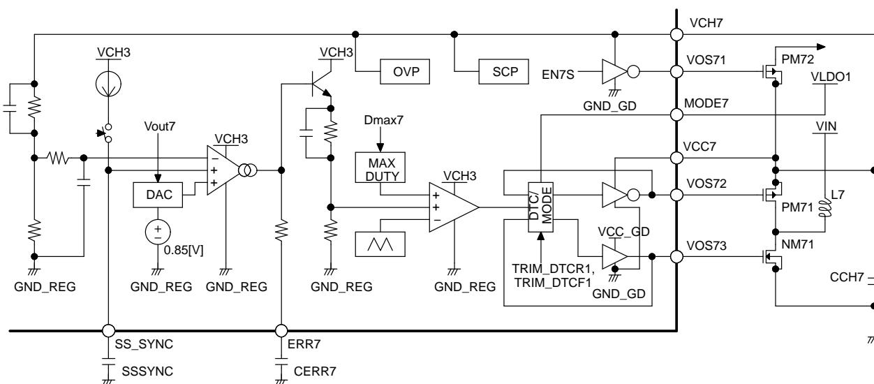
Figure 23. CH-7 Block Diagram (Step-up)
