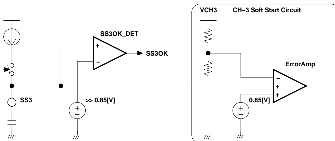
Figure 28. CH-3 Soft-Start Circuit
