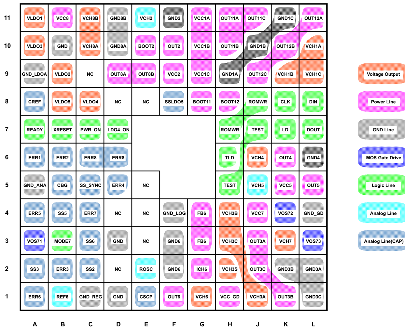
Figure 15. Pin Layout
