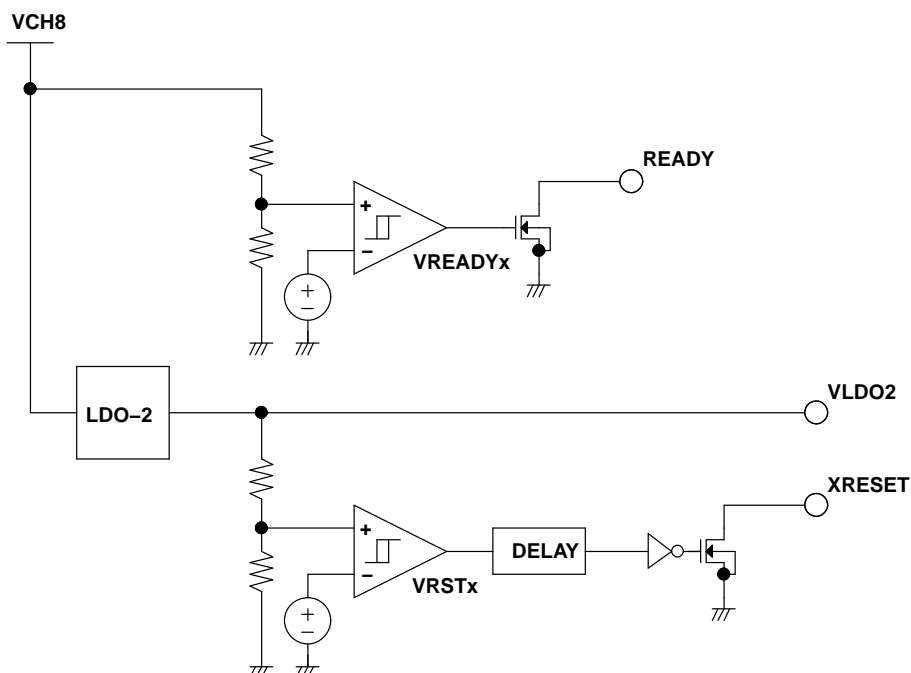
Figure 27. Sub-CPU Control Block Diagram
