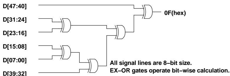
Figure 31. Configuration for Parity Bit Calculation
