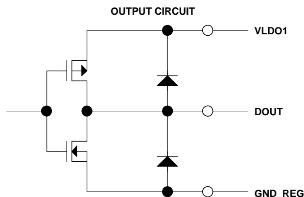
Figure 6. DOUT
