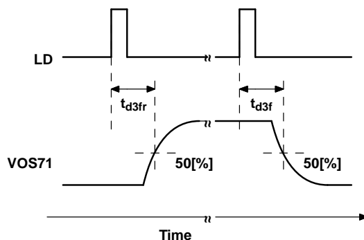
Figure 10. t_{d3r} and t_{d3f} Measurement References
