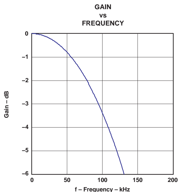
Figure 51. DSD Filter-4, Low BW
