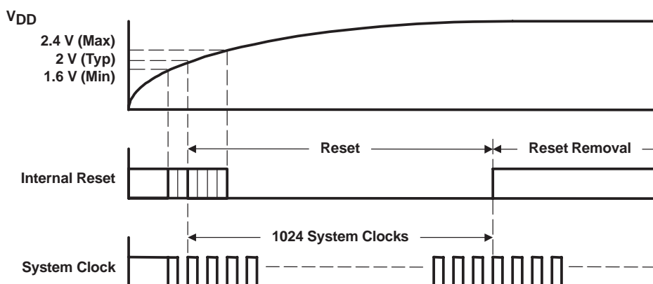
Figure 24. Power-On Reset Timing
