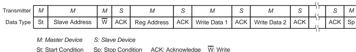
Figure 32. Write Operation
