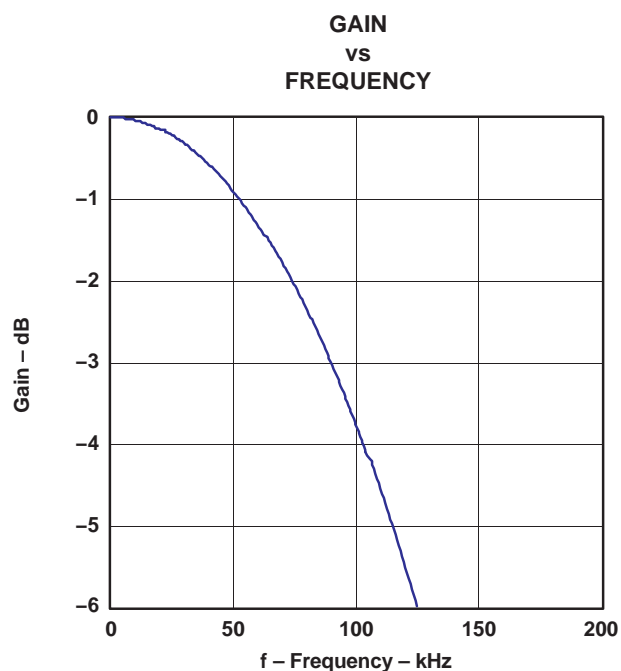
Figure 47. DSD Filter-2, Low BW
