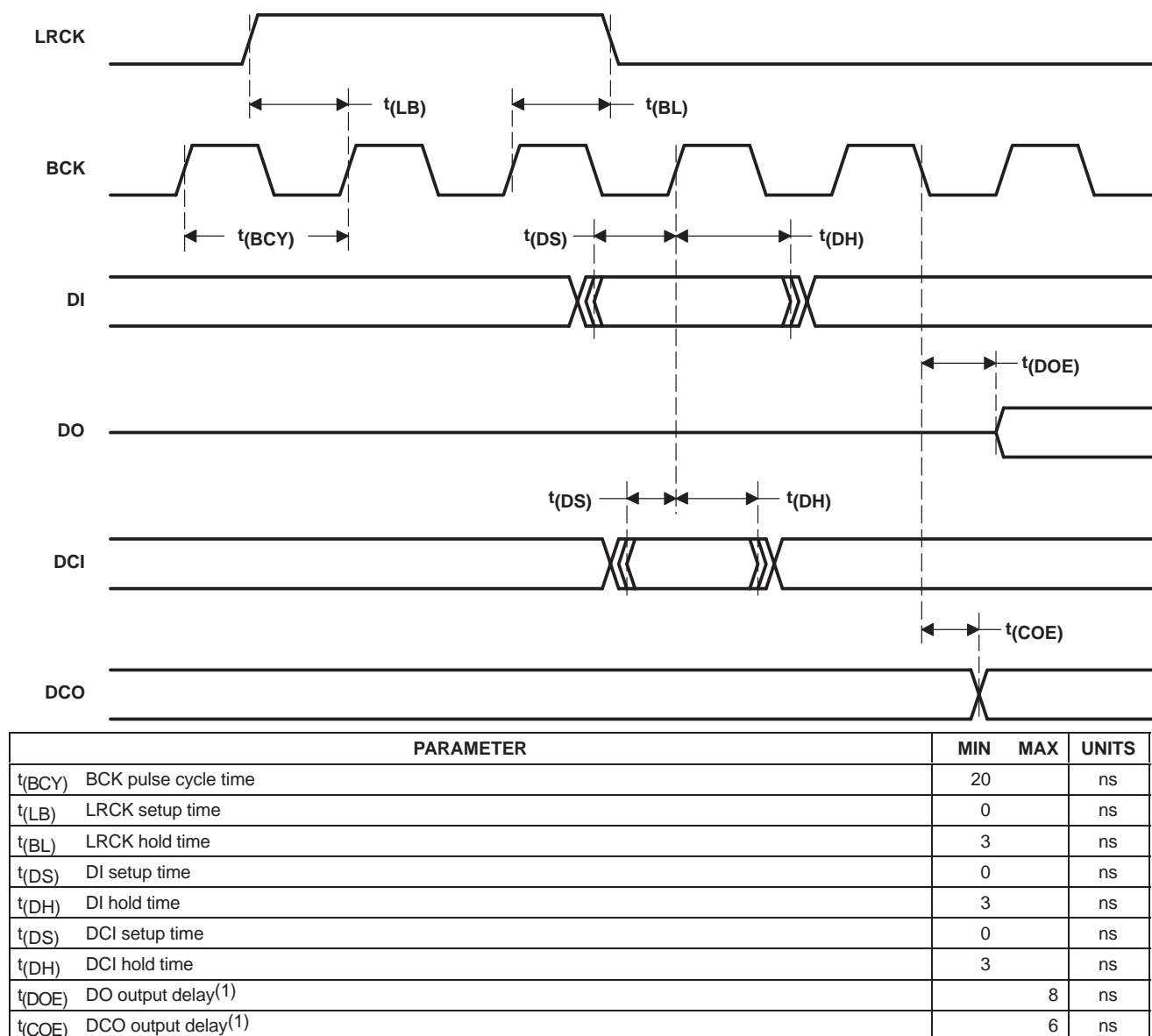
Figure 63. AC Timing of Daisy Chain Signals
