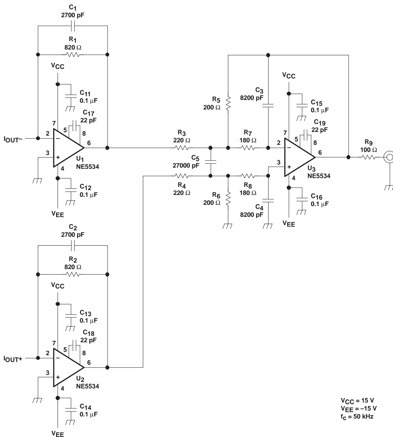
Figure 36. Measurement Circuit for PCM
