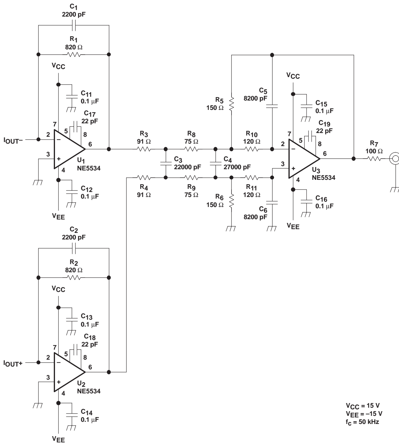
Figure 37. Measurement Circuit for DSD
