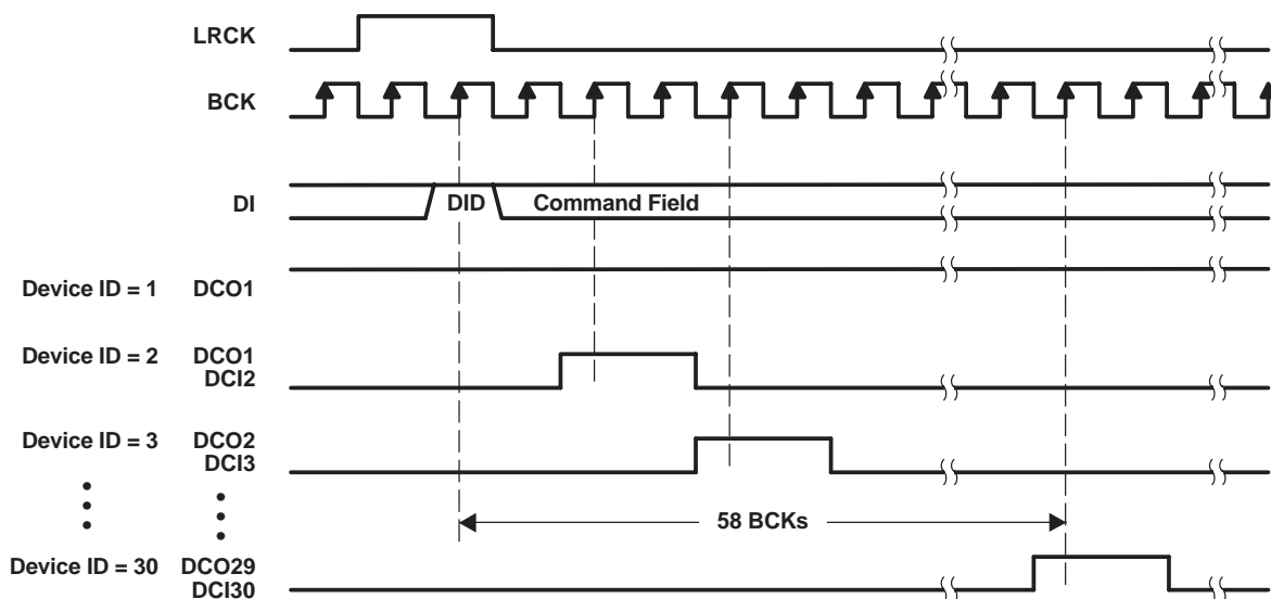
Figure 56. Device ID Determination Sequence
