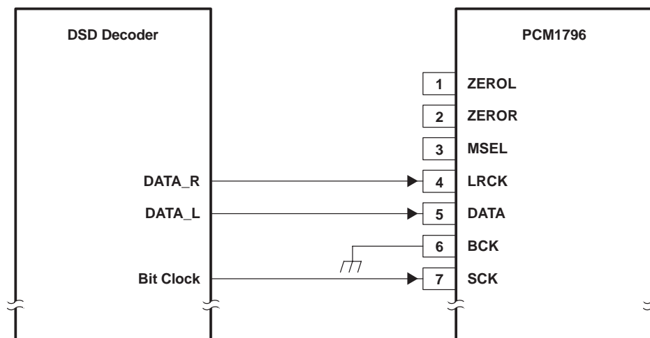
Figure 42. Connection Diagram in DSD Mode
