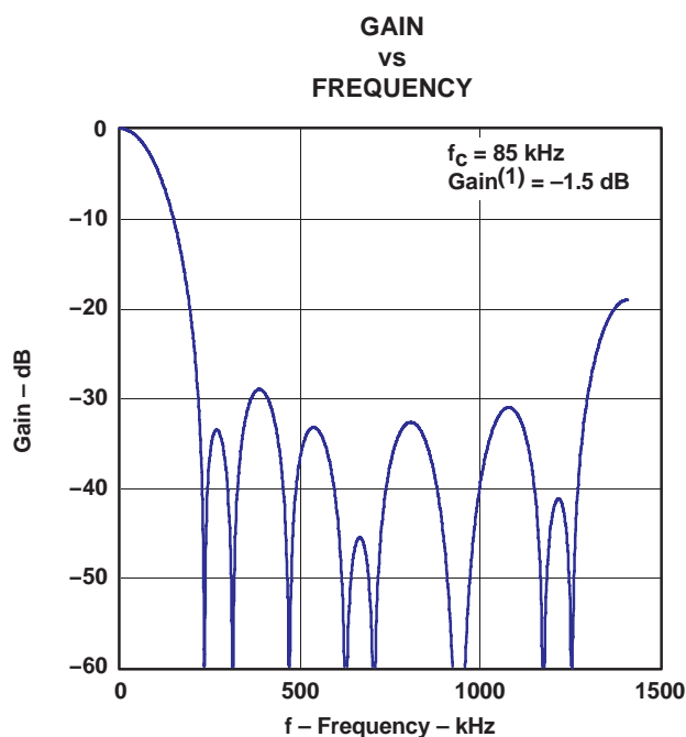
Figure 50. DSD Filter-3, High BW
