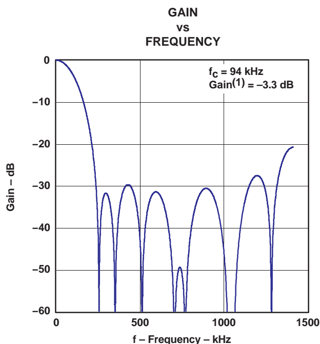
Figure 52. DSD Filter-4, High BW
