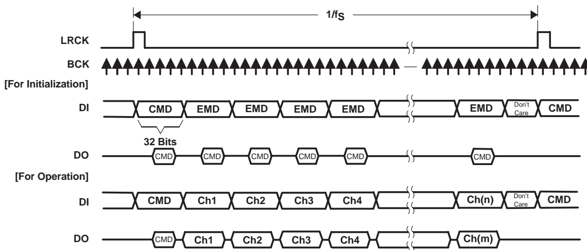
Figure 57. General TDMCA Frame
