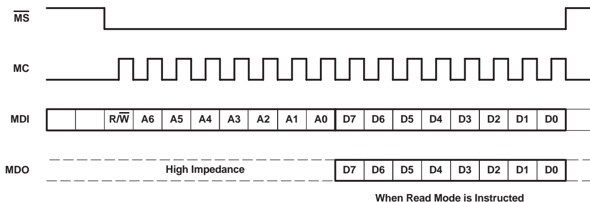
Figure 28. Control Data Word Format for MDI
