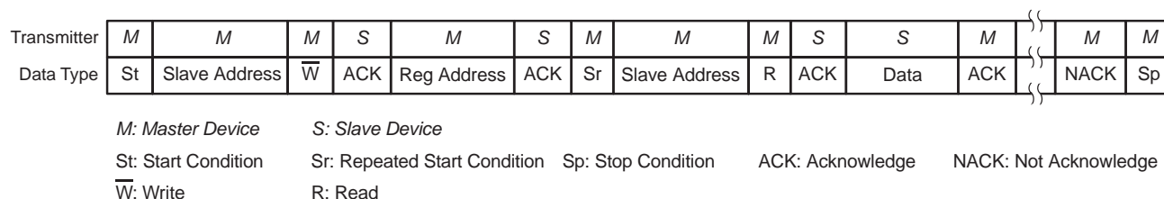
Figure 33. Read Operation
