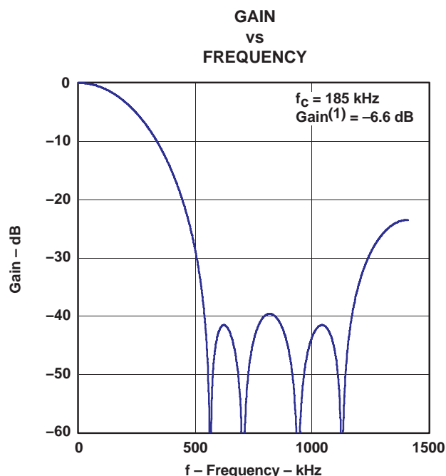
Figure 46. DSD Filter-1, High BW
