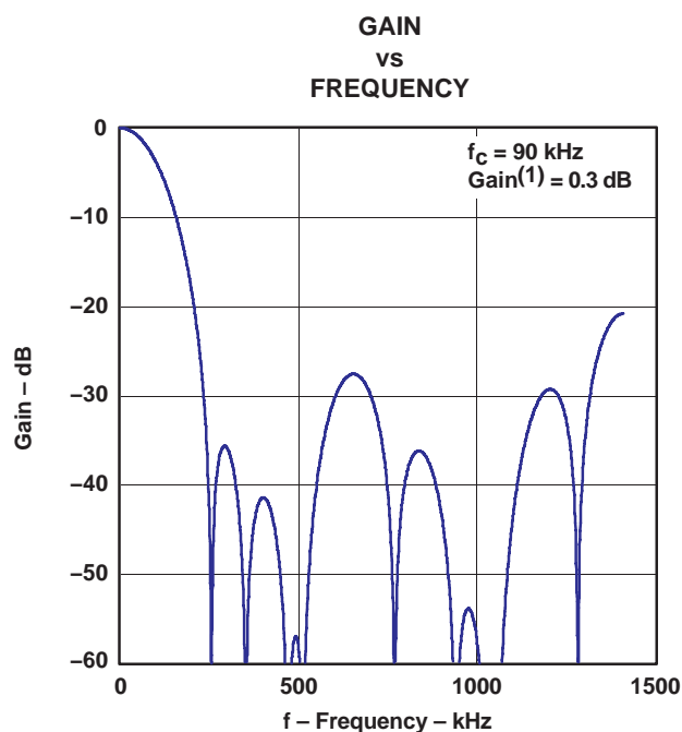
Figure 48. DSD Filter-2, High BW
