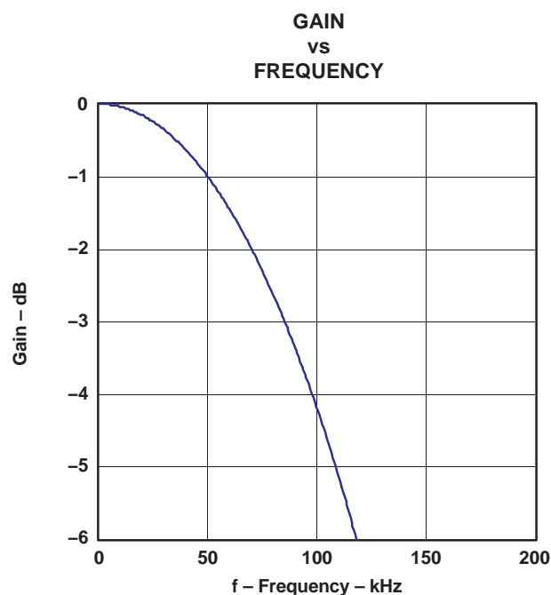
Figure 49. DSD Filter-3, Low BW
