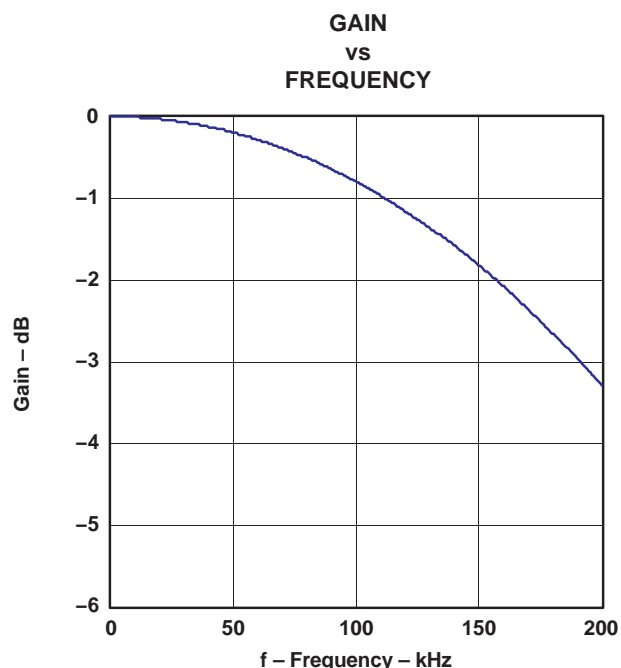
Figure 45. DSD Filter-1, Low BW
