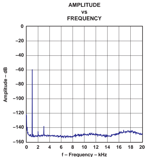
Figure 20. -60-dB Output Spectrum, BW = 100 kHz
