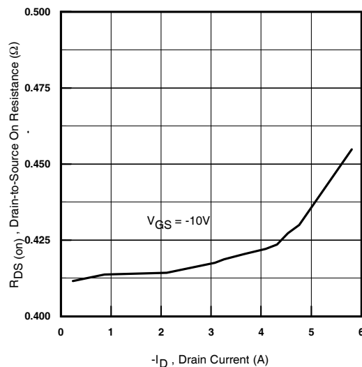
Fig 32. Typical On-Resistance Vs. Drain Current
