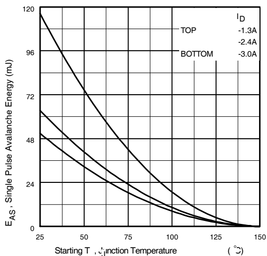
Fig 35a. Maximum Avalanche Energy Vs. Drain Current
