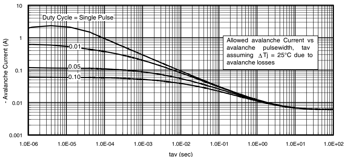
Fig 38. Typical Avalanche Current Vs. Pulsewidth
