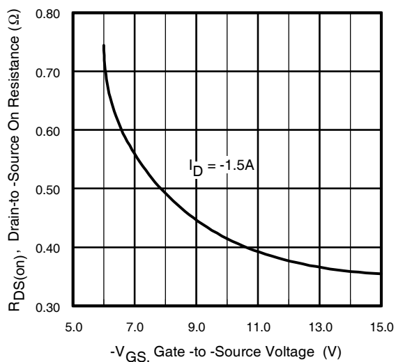
Fig 31. Typical On-Resistance Vs. Gate Voltage
