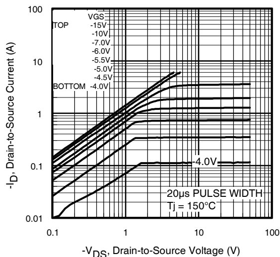
Fig 22. Typical Output Characteristics
