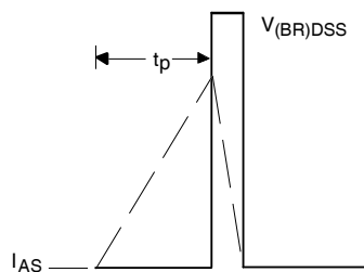
Fig 35d. Unclamped Inductive Waveforms
