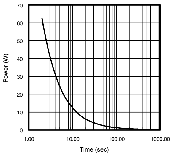
Fig 34. Typical Power Vs. Time
