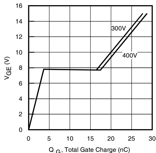
Fig. 17 - Typical Gate Charge vs. V_{GE} I_{CE} = 8.0A ; L = 600\mu H
