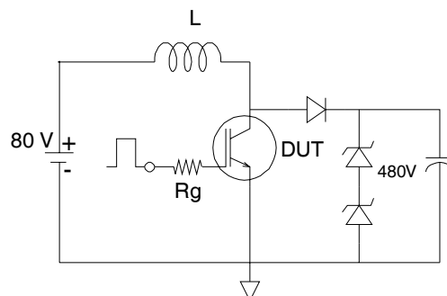
Fig.C.T.2 - RBSOA Circuit
