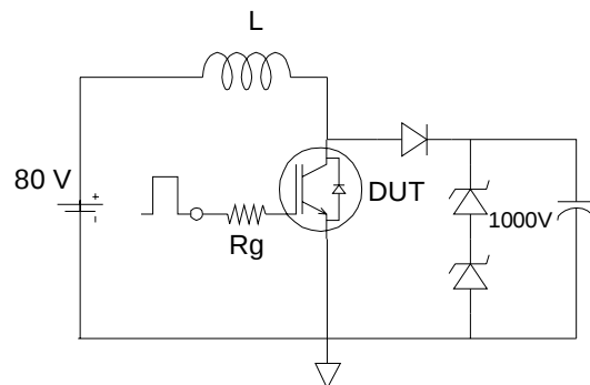
Fig.C.T.2 - RBSOA Circuit
