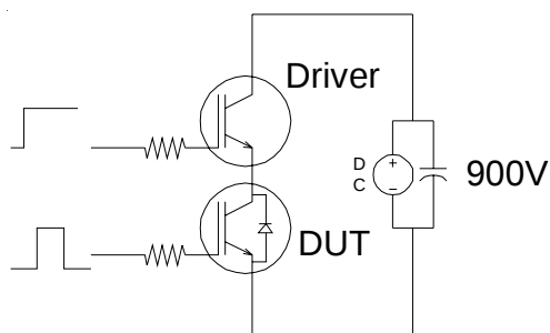
Fig.C.T.3 - RBSOA Circuit
