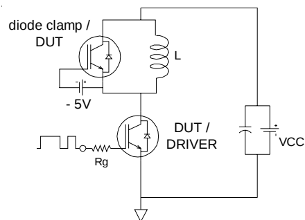
Fig.C.T.4 - RBSOA Circuit
