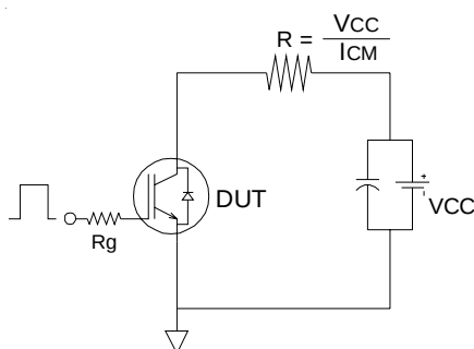
Fig.C.T.5 - RBSOA Circuit
