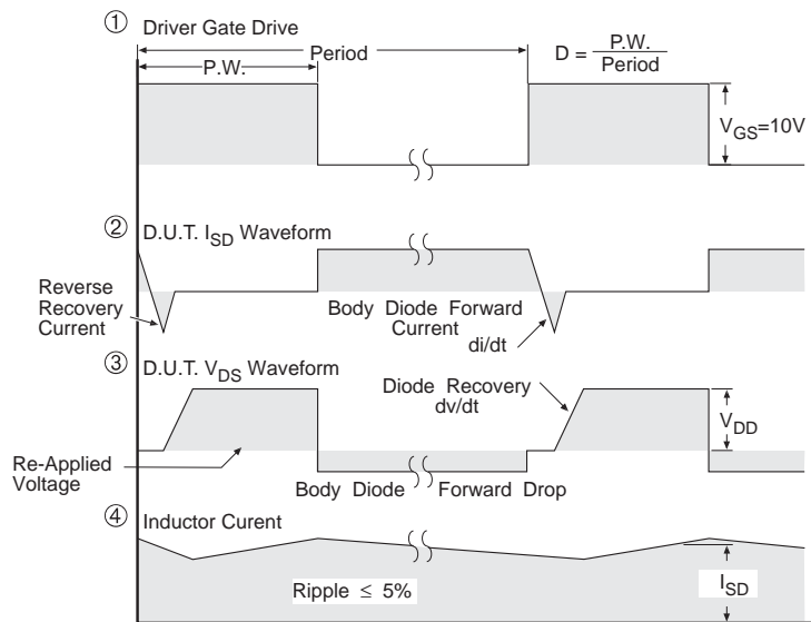
Fig 13. For N-channel HEXFET® power MOSFET s
