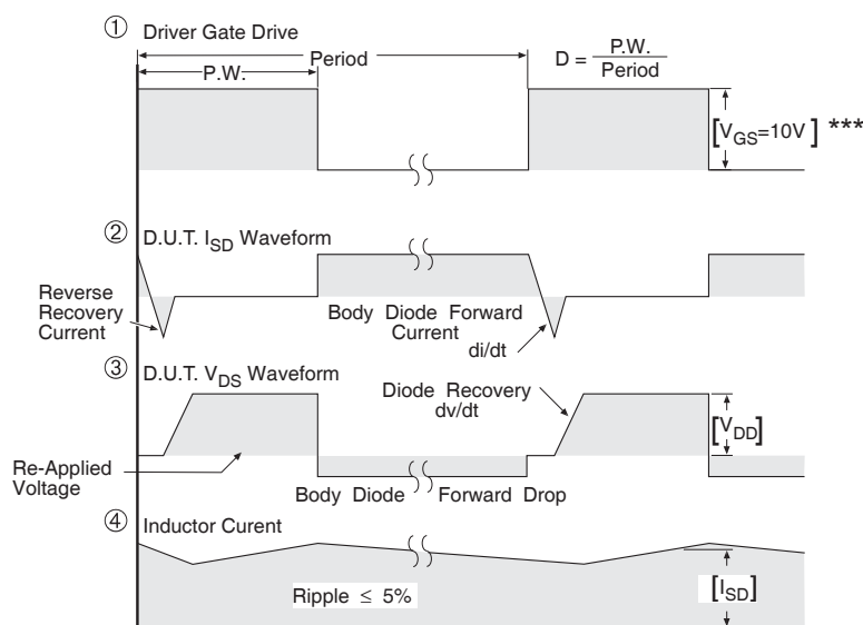
Fig 13. For P-channel HEXFET® power MOSFET s
