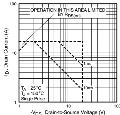
Fig 19. Maximum Safe Operating Area
