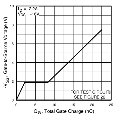
Fig 17. Typical Gate Charge Vs. Gate-to-Source Voltage
