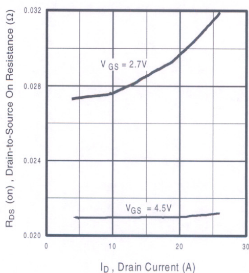
Fig 6. Typical On-Resistance Vs. Drain Current
