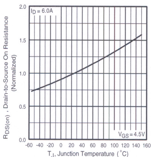
Fig 5. Normalized On-Resistance Vs. Temperature
