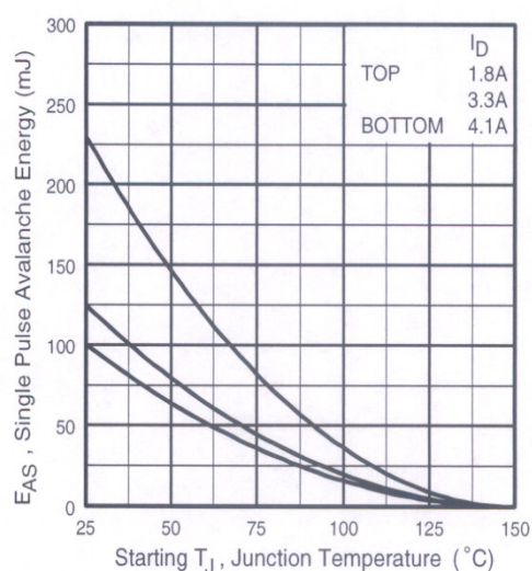
Fig 8. Maximum Avalanche Energy Vs. Drain Current
