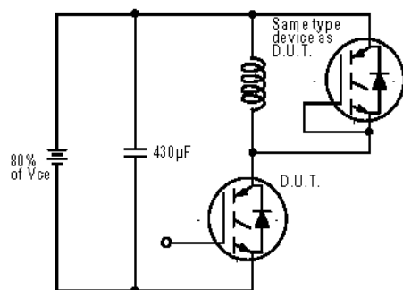
Fig. 18a - Test Circuit for Measurement of I_{LM} , E_{on} , E_{off}(\text{diode}) , t_{tr} , Q_{tr} , I_{tr} , t_{d(on)} , t_r , t_{d(off)} , t_f
