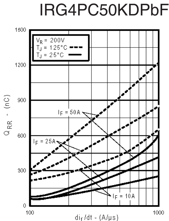
Fig. 16 - Typical Stored Charge vs. di_f/dt
