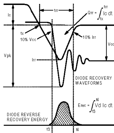
Fig. 18d - Test Waveforms for Circuit of Fig. 18a, Defining E_{rec} , t_{tr} , Q_{tr} , I_{tr}
