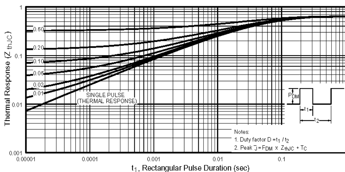
Fig. 6 - Maximum Effective Transient Thermal Impedance, Junction-to-Case
