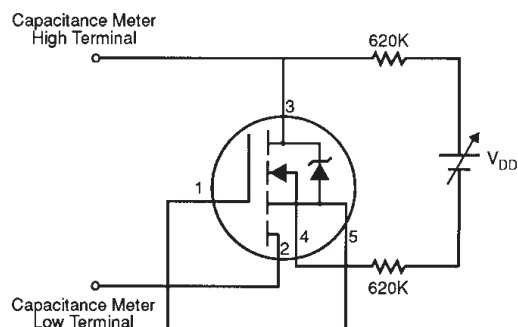
Fig. 19 HEXSense Sensing Cell Output Capacitance Test Circuit
