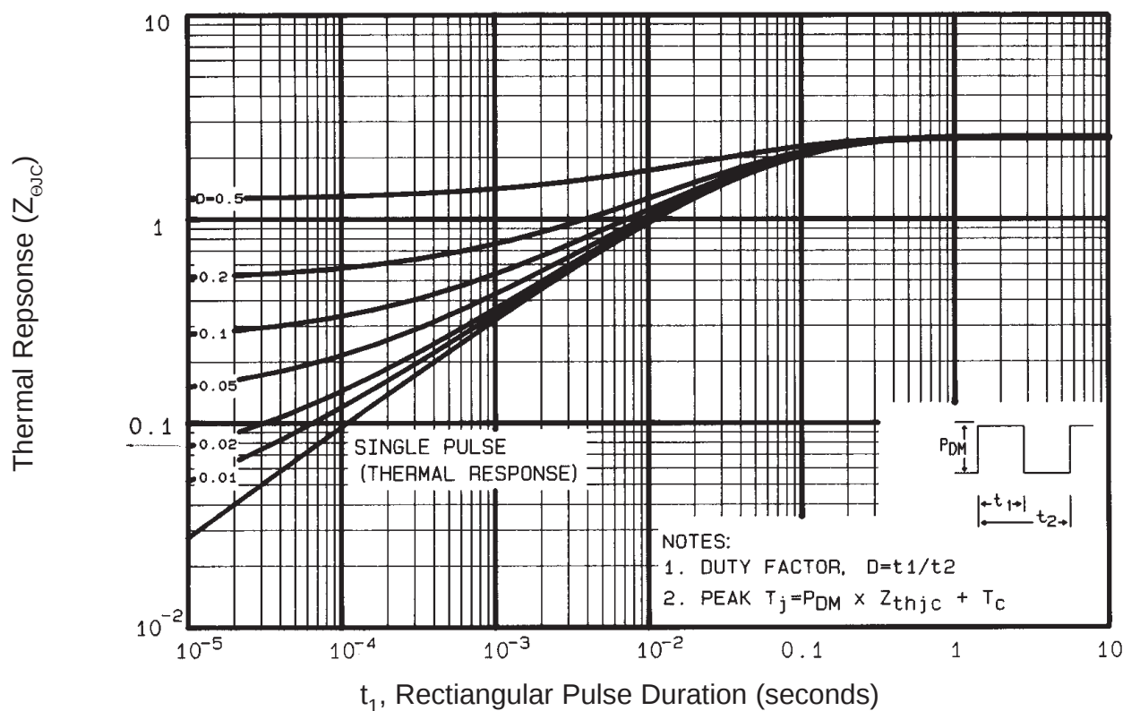
Fig. 11 Maximum Effective Transient Thermal Impedance, Junction-to-Case
