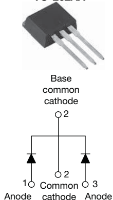
VS-MBR25..CT-1PbF
