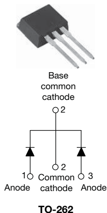
VS-MBR20..CT-1PbF
