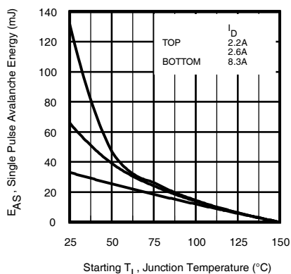
Fig 23. Maximum Avalanche Energy vs. Drain Current
