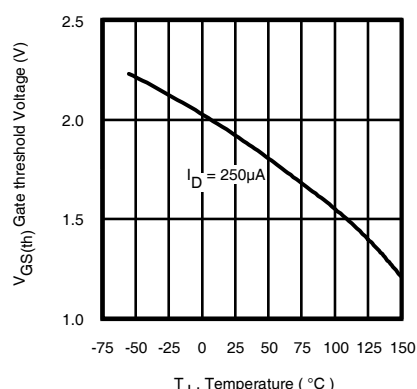
Fig 22. Threshold Voltage vs. Temperature
