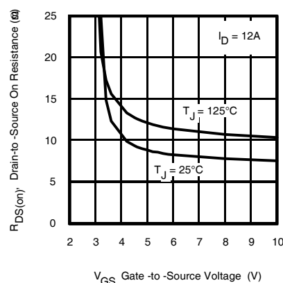
Fig 18. Typical On-Resistance vs. Gate Voltage
