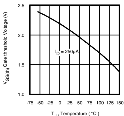
Fig 21. Threshold Voltage vs. Temperature
