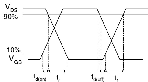
Fig 29. Switching Time Waveforms
