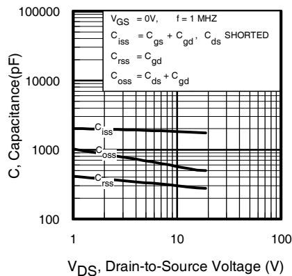
Fig 8. Typical Capacitance Vs.Drain-to-Source Voltage
