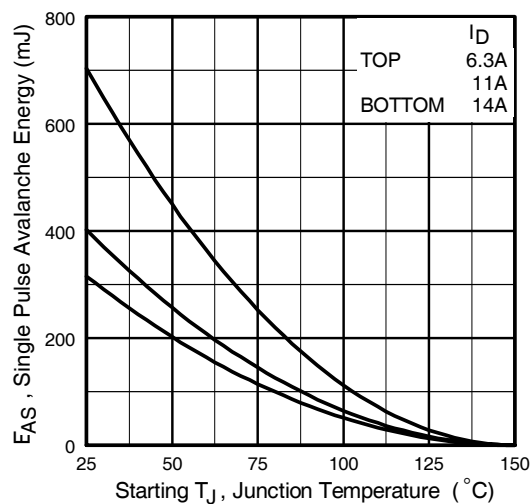
Fig 15c. Maximum Avalanche Energy Vs. Drain Current
