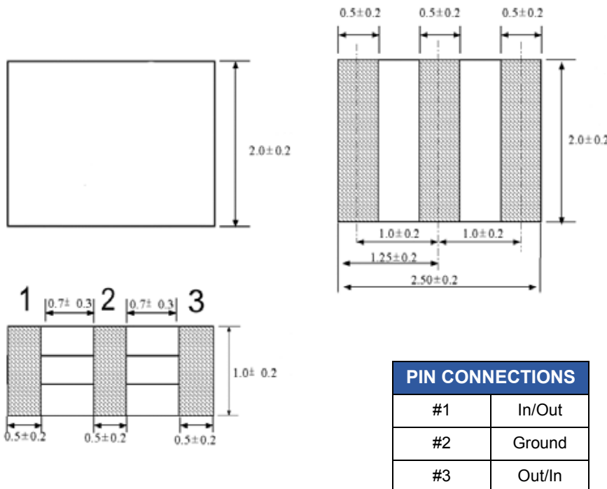
Figure 1) ECS-HFR-B Series - Top, Side and Bottom Views
