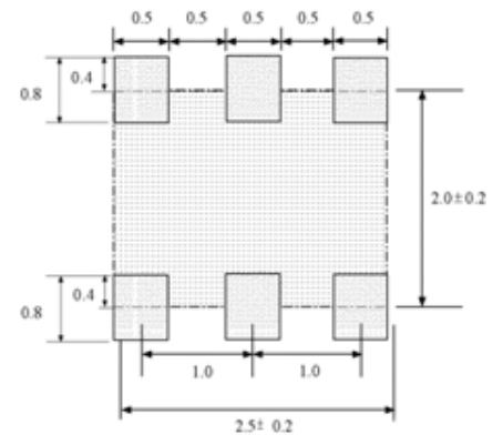
Figure 2) Land Pattern
