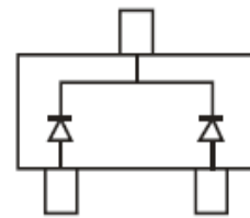
BAS40-05T Marking: 45
