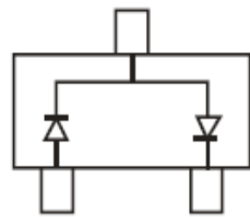
BAS40-04T Marking: 44
