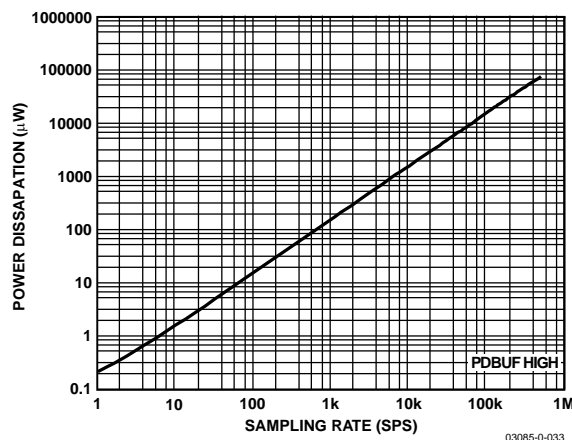
Figure 31. Power Dissipation vs. Sample Rate
