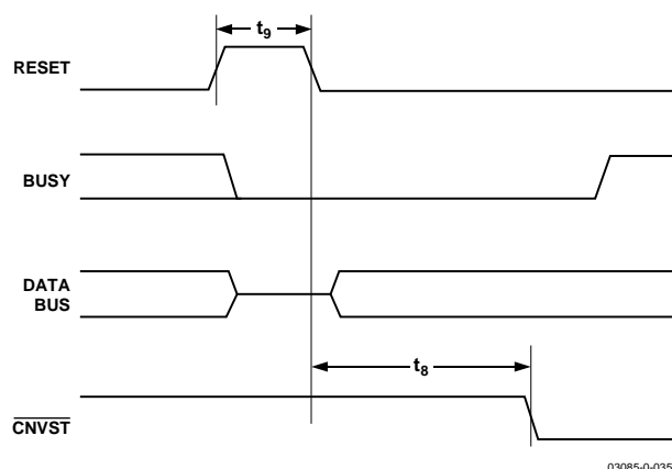
Figure 33. RESET Timing
