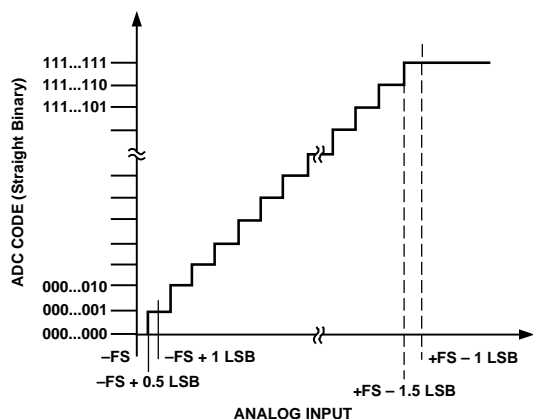
Figure 24. ADC Ideal Transfer Function
