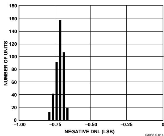
Figure 12. Typical Negative DNL Distribution (424 Units)
