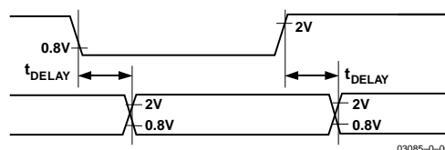
Figure 3. Voltage Reference Levels for Timing
