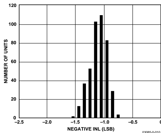
Figure 10. Typical Negative INL Distribution (424 Units)
