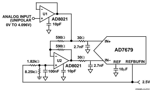
Figure 29. Single-Ended-to-Differential Driver Circuit (Internal Reference Buffer Used)
