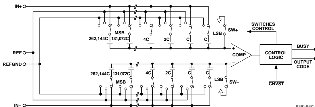
Figure 23. ADC Simplified Schematic
