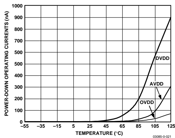
Figure 20. Power-Down Operating Currents vs. Temperature
