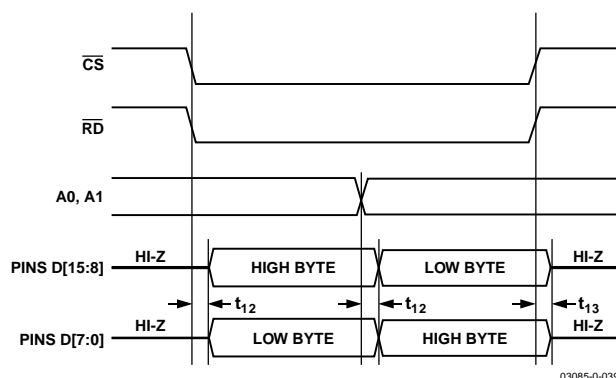
Figure 37. 8-Bit and 16-Bit Parallel Interface
