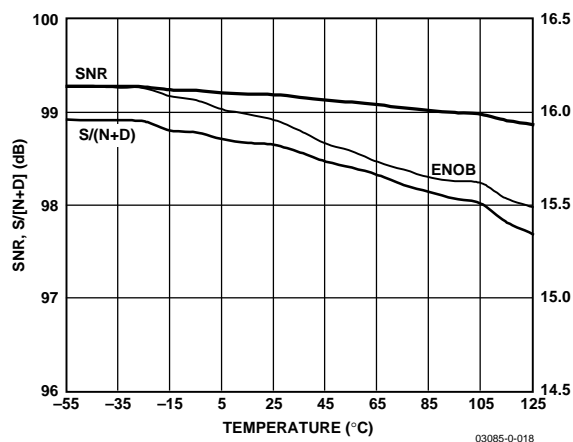
Figure 17. SNR, S/(N+D), and ENOB vs. Temperature
