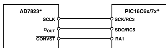
Figure 17. Interfacing to the PIC16/PIC17
