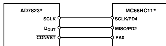
Figure 18. Interfacing to the MC68HC11
