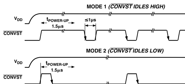
Figure 12. Power-Up Times
