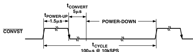
Figure 13. Automatic Power-Down
