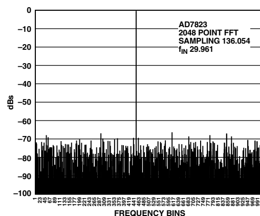
Figure 3. AD7823 SNR
