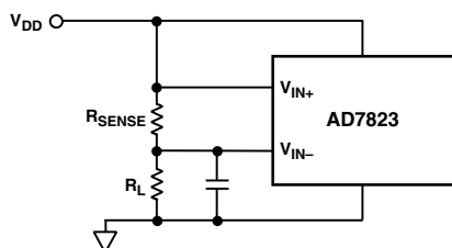
Figure 9. DC Current Measurement Scheme
