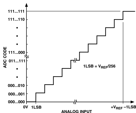
Figure 11. Transfer Characteristic
