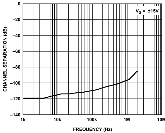
Figure 27. Channel Separation
