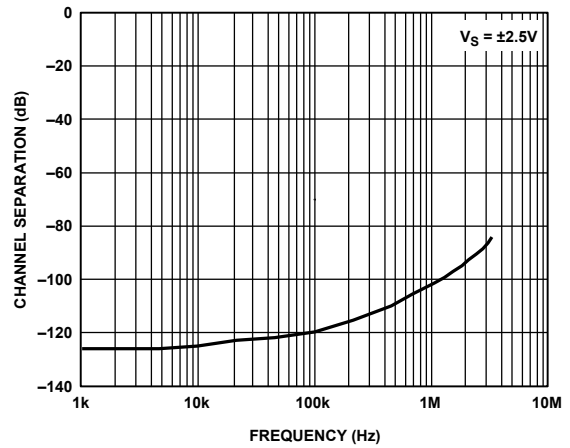
Figure 48. Channel Separation
