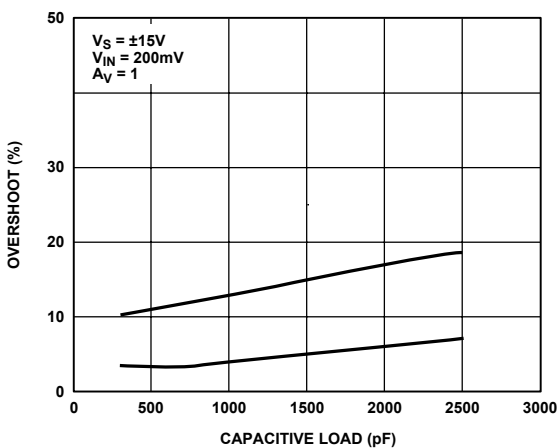
Figure 10. Overshoot vs. Load Capacitance
