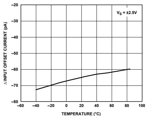
Figure 43. Δ Input Bias Current vs. Temperature
