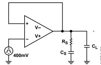
Figure 51. Snubber Network
