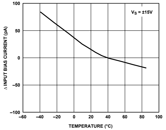
Figure 24. Δ Input Bias Current vs. Temperature
