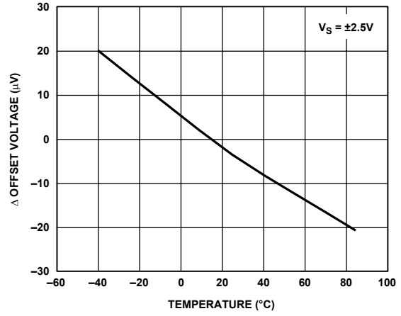
Figure 41. Δ Offset Voltage vs. Temperature
