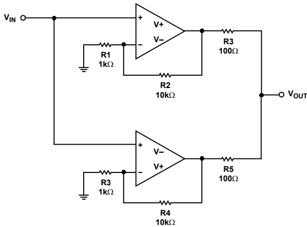
Figure 55. Paralleling Amplifiers
