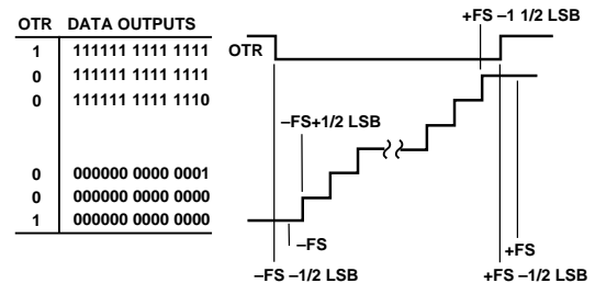
Figure 42. Output Data Format
