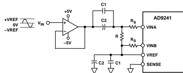
Figure 34. AC-Coupled Input
