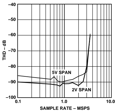
Figure 8. THD vs. Sample Rate ( f_{\text{IN}} = 0.3 \text{ MHz} , A_{\text{IN}} = -0.5 \text{ dBFS} , V_{\text{CM}} = 2.5 \text{ V} )
