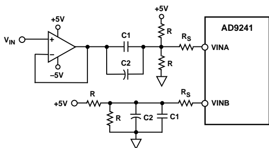
Figure 35. AC-Coupled Input-Flexible Input Span, V CM = 2.5 V
