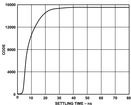
Figure 23. Settling Time
