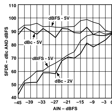
Figure 9. Single Tone SFDR ( f_{\text{IN}} = 0.6 \text{ MHz} , V_{\text{CM}} = 2.5 \text{ V} )
