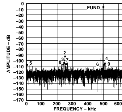
Figure 7. Typical FFT, f_{\text{IN}} \cong 500 \text{ kHz} (Input Span = 2 V, V_{\text{CM}} = 2.5 \text{ V} )
