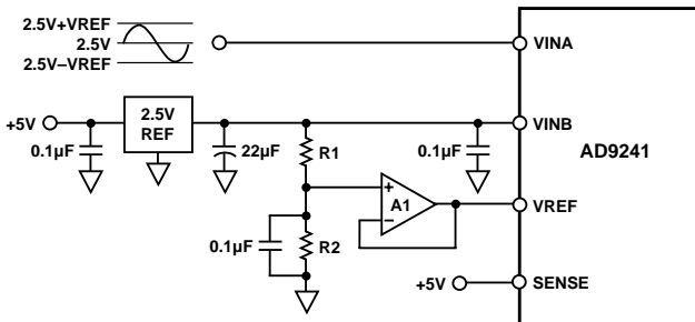
Figure 39. External Reference, V_{CM} = 2.5 V (2.5 V on VINB, Resistor Divider to Make VREF)
