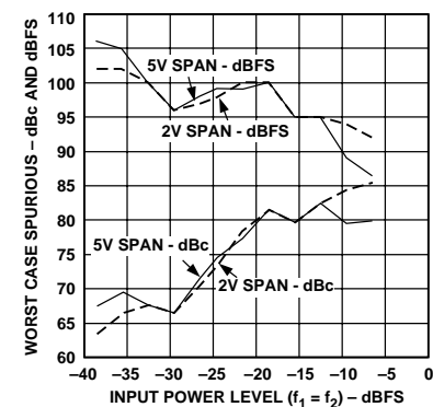
Figure 10. Dual Tone SFDR ( f_1 = 0.5 \text{ MHz} , f_2 = 0.6 \text{ MHz} , V_{\text{CM}} = 2.5 \text{ V} )
