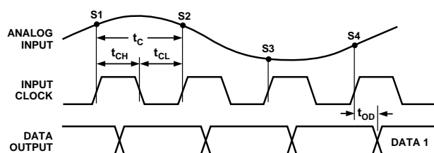
Figure 1. Timing Diagram
