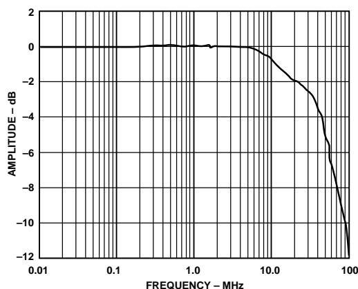
Figure 22. Full-Power Bandwidth
