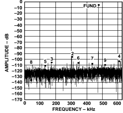
Figure 4. Typical FFT, f_{\text{IN}} \cong 500 \text{ kHz} (Input Span = 5 V, V_{\text{CM}} = 2.5 \text{ V} )
