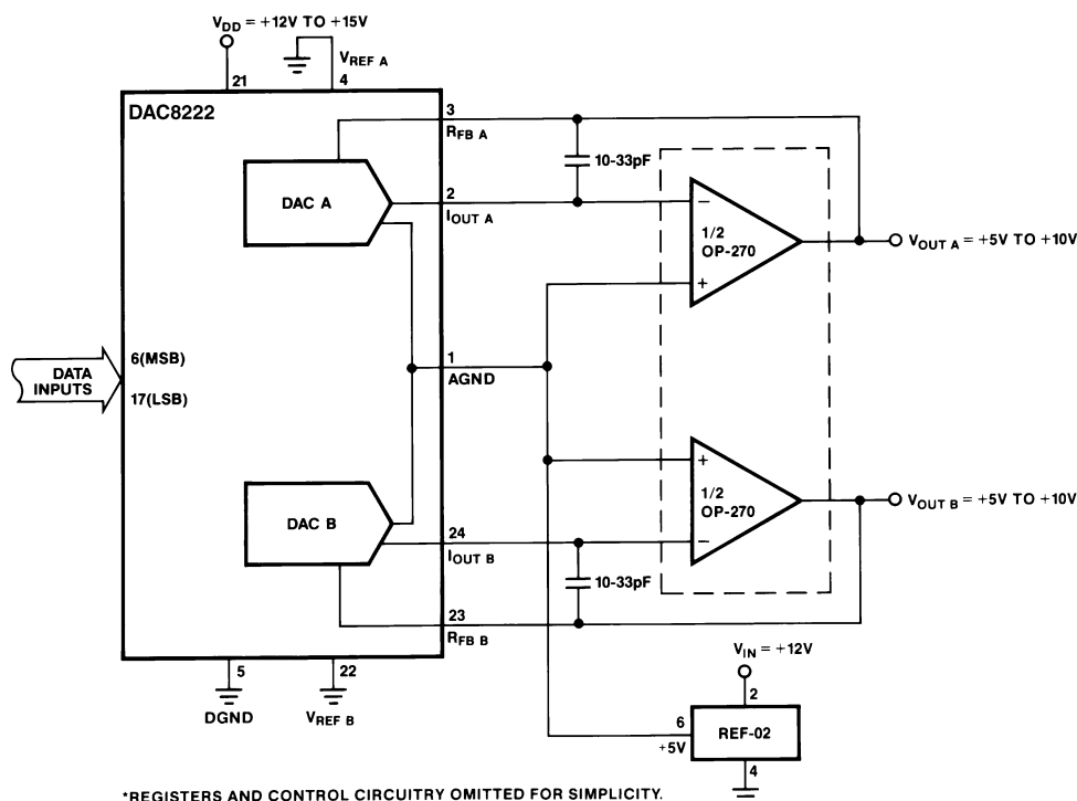
Figure 26. Single Supply Operation (Current Switching Mode)
