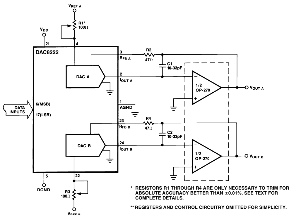
Figure 24. Unipolar Configuration (Two-Quadrant Multiplication)
