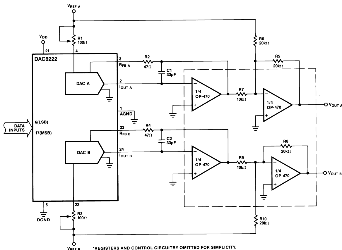
Figure 25. Bipolar Configuration (Four-Quadrant Multiplication)
