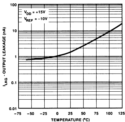
Figure 15. Output Leakage Current vs. Temperature
