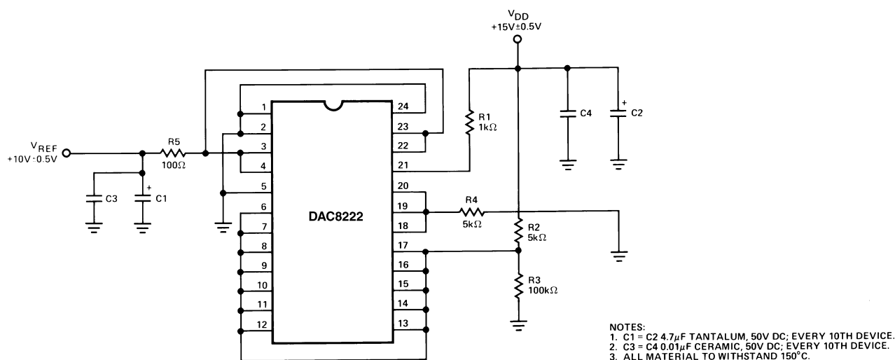
Figure 18. Burn-In Circuit
