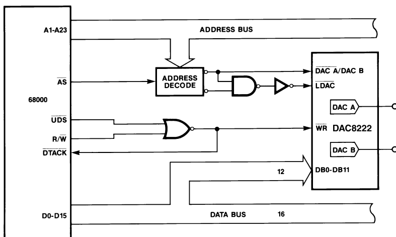
Figure 30. DAC8222 to 68000 Interface
