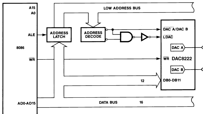
Figure 29. DAC8222 to 8086 Interface
