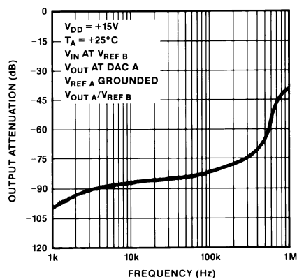
Figure 16. Analog Crosstalk vs. Frequency
