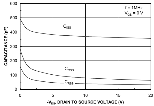
Figure 8. Capacitance Characteristics.
