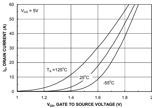
Figure 5. Transfer Characteristics.
