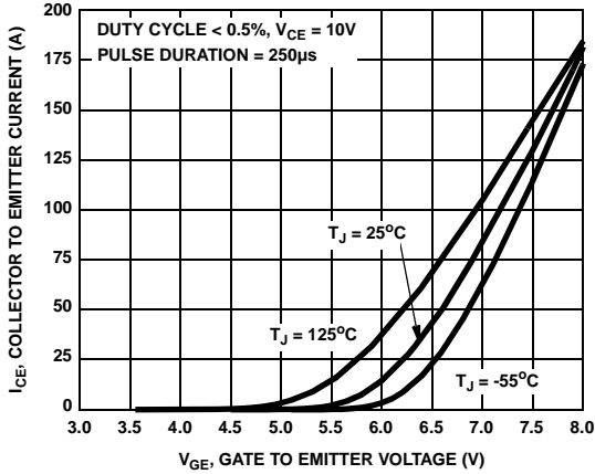
Figure 13. Transfer Characteristic
