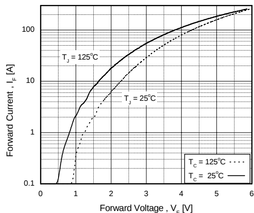
Figure 17. Forward Characteristics
