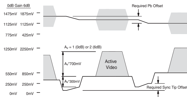
Figure 1. Bi-Level Sync Tip Clamping and Bias
