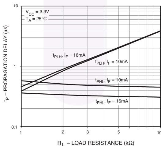
Fig. 9 Propagation Delay vs. Load Resistance
