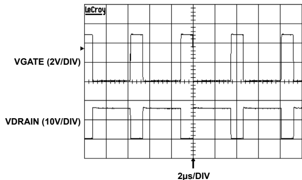
FIGURE 13. GATE AND DRAIN WAVEFORMS VOUT = 14.0V
