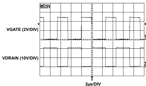
FIGURE 12. GATE AND DRAIN WAVEFORMS VOUT = 19.0V
