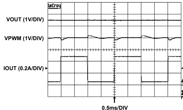
FIGURE 11. DYNAMIC RESPONSE VOUT = 14.0V
