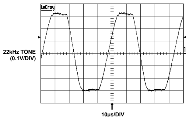
FIGURE 6. 22kHz TONE
