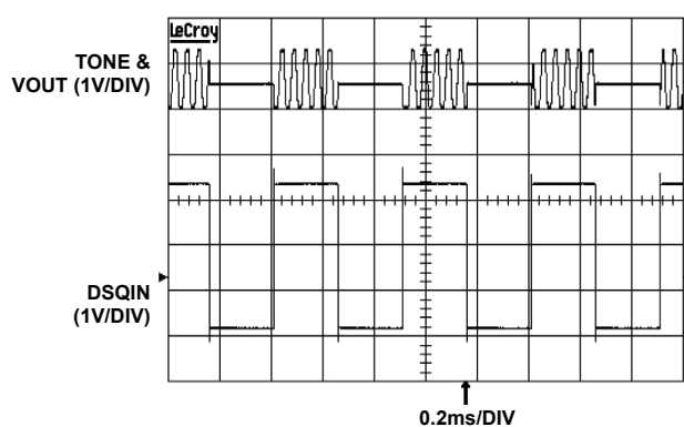
FIGURE 7. 22kHz TONE MODULATED BY DSQIN
