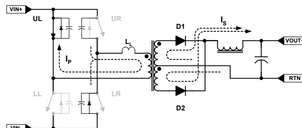
FIGURE 16. UPPER SWITCH TOGGLE AND RESONANT TRANSITION
