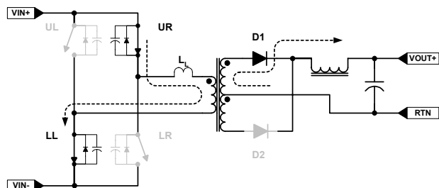
FIGURE 14. UR - LL POWER TRANSFER
