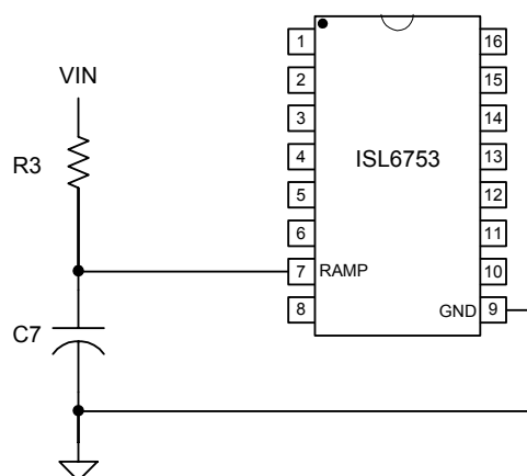
FIGURE 6. VOLTAGE FEED FORWARD CONTROL
