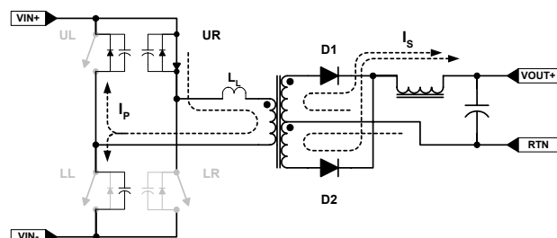
FIGURE 15. UR - UL FREE-WHEELING PERIOD
