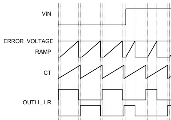
FIGURE 5. VOLTAGE FEED FORWARD BEHAVIOR
