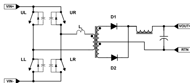
FIGURE 10. IDEALIZED FULL-BRIDGE
