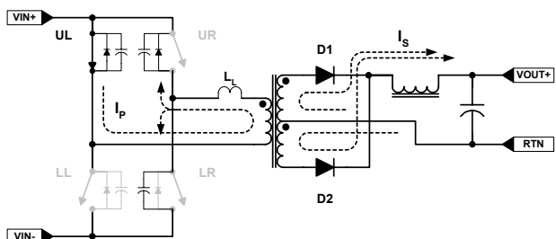
FIGURE 12. UL - UR FREE-WHEELING PERIOD
