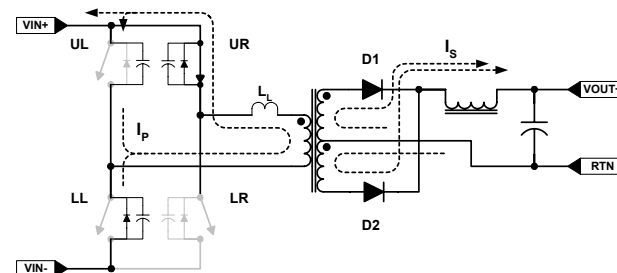
FIGURE 13. UPPER SWITCH TOGGLE AND RESONANT TRANSITION
