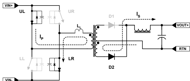
FIGURE 11. UL - LR POWER TRANSFER CYCLE
