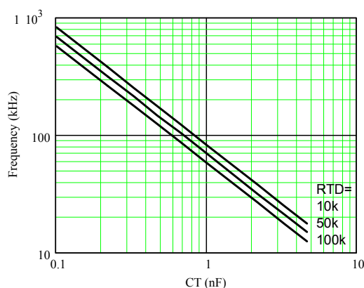
FIGURE 4. CAPACITANCE vs FREQUENCY
