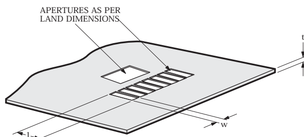
Figure 14. Solder stencil aperture.
