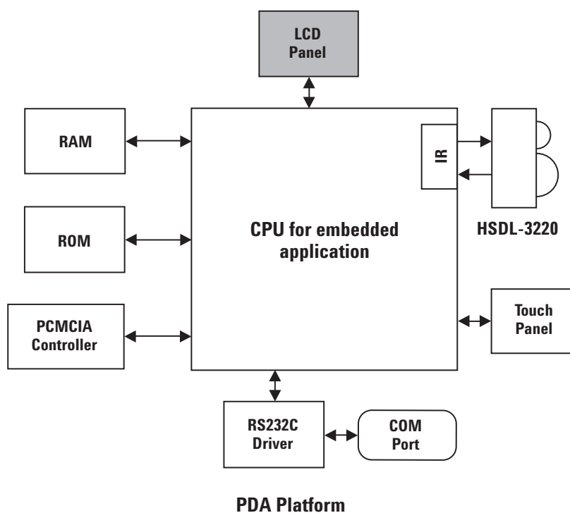
Figure 18. PDA platform.
