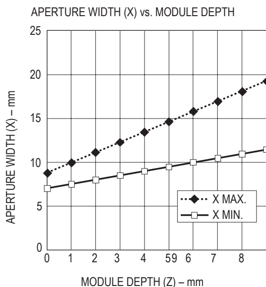
Figure 20. Aperture width (X) vs. module depth.
