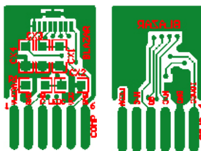
Figure 16. PCB layout suggestion.
