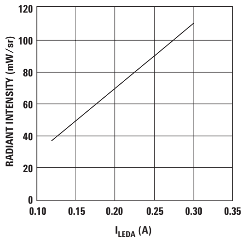
Figure 9. Radiant Intensity vs I_{LEDA} .
