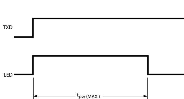
Figure 7. TxD "Stuck On" protection waveform.
