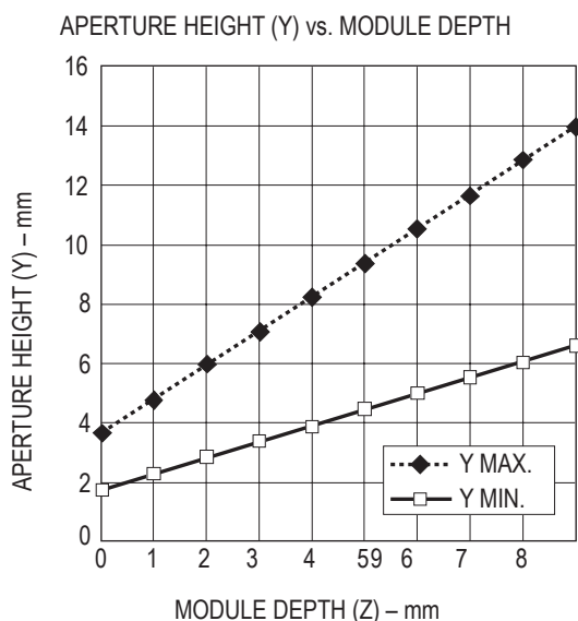
Figure 21. Aperture height (Y) vs. module depth.
