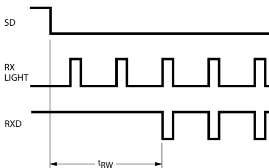
Figure 8. Receiver wakeup time waveform.
