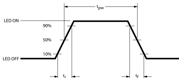
Figure 6. LED optical waveform.
