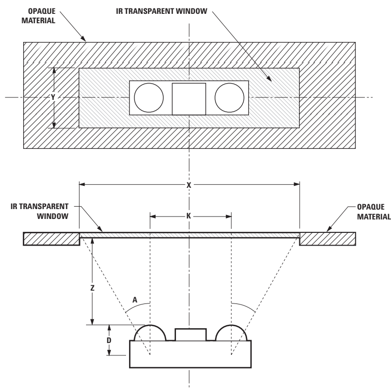
Figure 19. Window design diagram.
