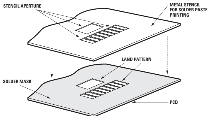
Figure 12. Stencil and PCBA.
