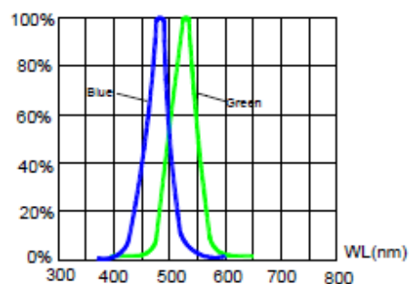
Relative Luminous Flux vs Wavelength
