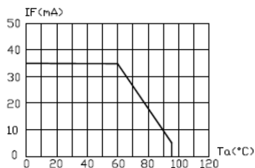
Maximum Forward DC Current vs Ambient Temperature
