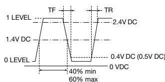
Figure 2) Output Wave Form
