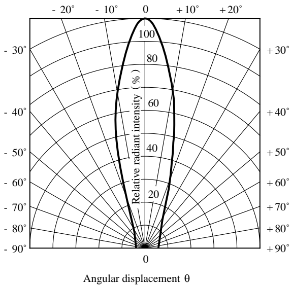
Fig. 9 Radiation Diagram
