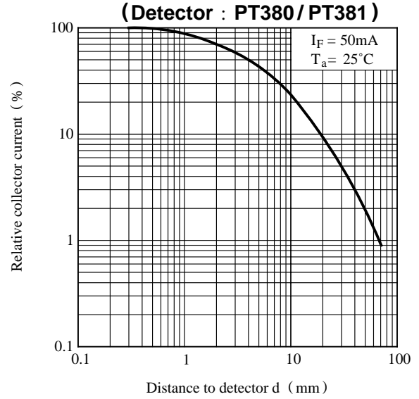
Fig. 8 Relative Collector Current vs. Distance
