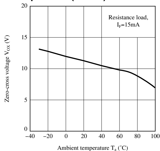
Fig.9 Zero-cross Voltage vs. Ambient Temperature (rank B)
