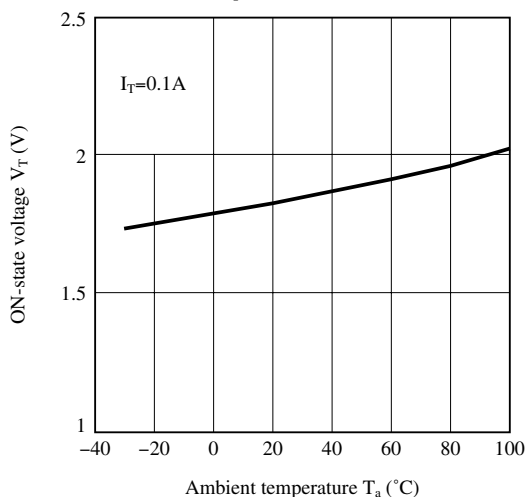
Fig.6 ON-state Voltage vs. Ambient Temperature
