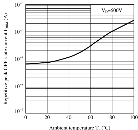
Fig.8 Repetitive Peak OFF-state Current vs. Ambient Temperature
