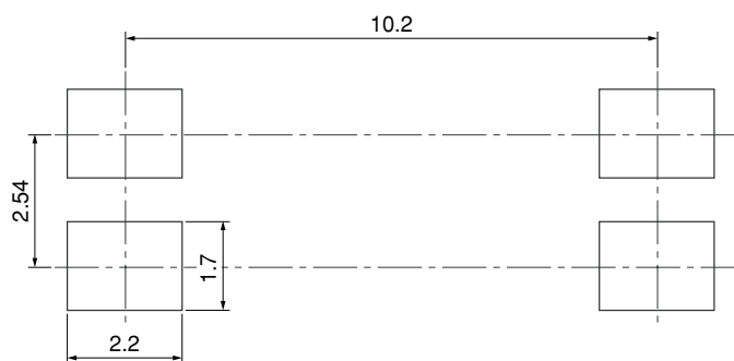
Wide SMT Gullwing Lead-form
