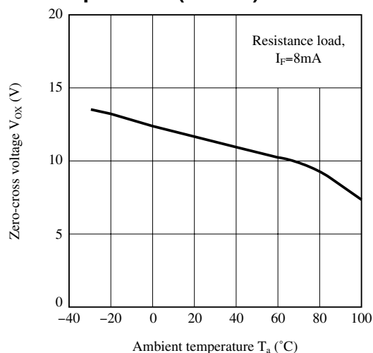
Fig.10 Zero-cross Voltage vs. Ambient Temperature (rank C)
