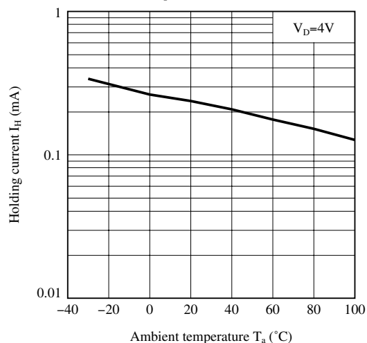
Fig.7 Holding Current vs. Ambient Temperature
