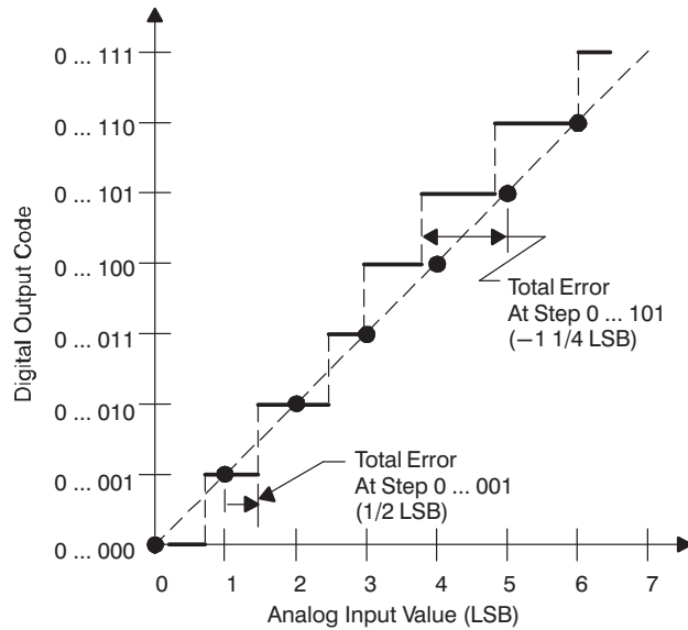
Figure 25. Absolute Accuracy (Total) Error
