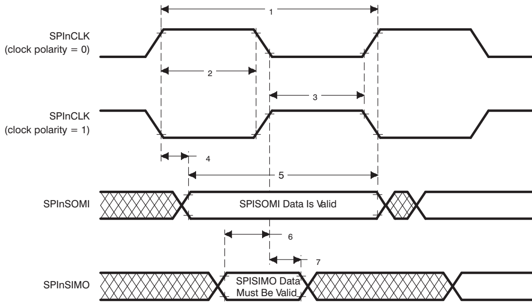
Figure 15. SPIn Slave Mode External Timing (CLOCK PHASE = 0)
