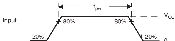
Figure 12. CMOS-Level Inputs
