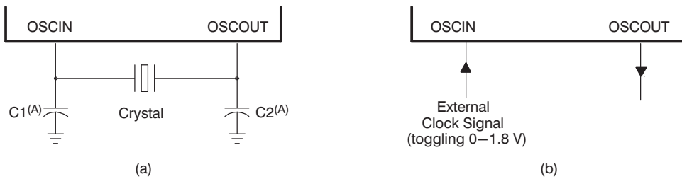
Figure 6. Crystal/Clock Connection
