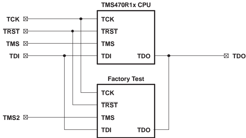
Figure 2. JTAG Interface
