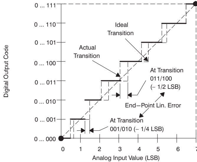
Figure 24. Integral Nonlinearity (INL) Error
