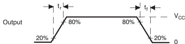
Figure 11. CMOS-Level Outputs
