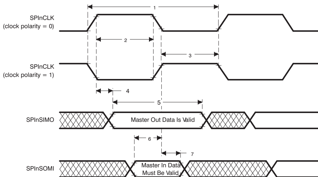
Figure 13. SPIn Master Mode External Timing (CLOCK PHASE = 0)
