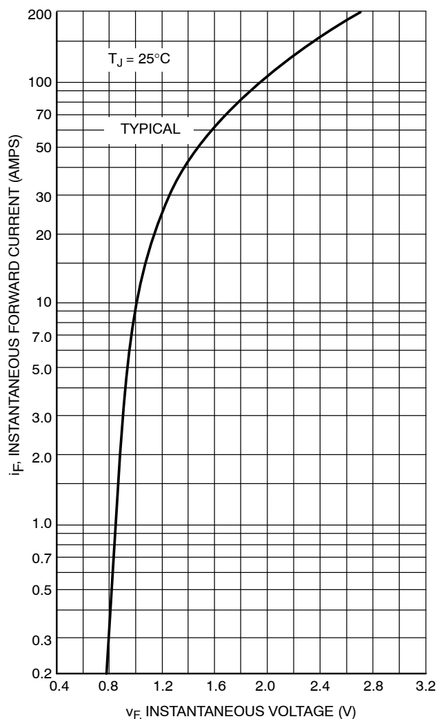
Figure 1. Forward Voltage
