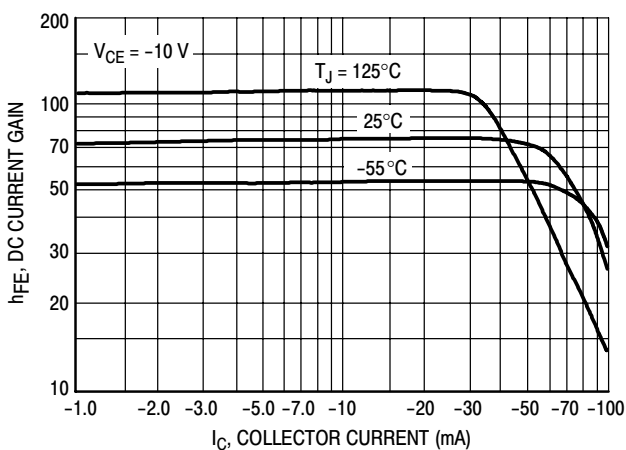
Figure 3. DC Current Gain PNP 2N6520
