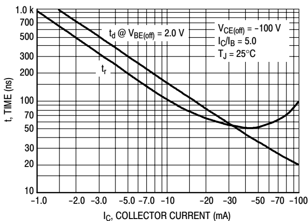
Figure 13. Turn-On Time PNP 2N6520
