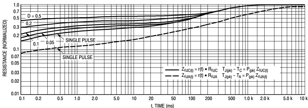
Figure 17. Thermal Response
