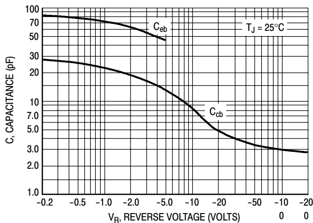
Figure 11. Capacitance PNP 2N6520
