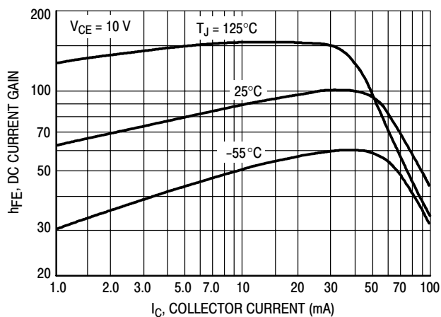
Figure 1. DC Current Gain NPN 2N6515
