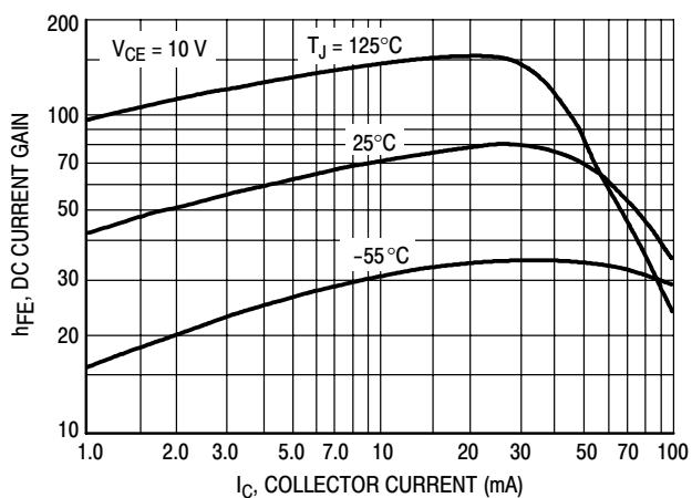
Figure 2. DC Current Gain NPN 2N6517
