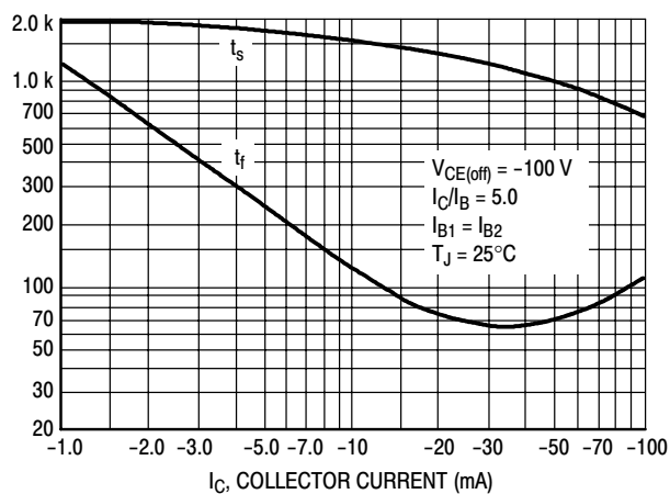
Figure 15. Turn-Off Time PNP 2N6520
