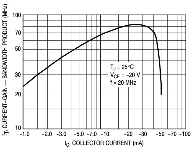
Figure 5. Current-Gain – Bandwidth Product PNP 2N6520
