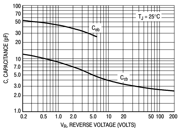
Figure 10. Capacitance NPN 2N6515, 2N6517
