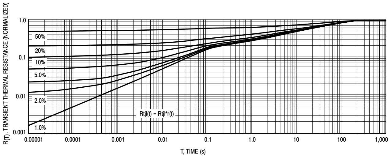
Figure 9. Thermal Response Junction to Ambient
