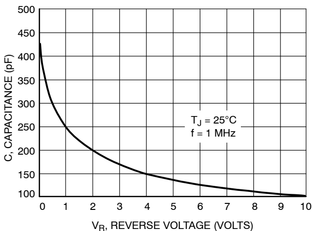
Figure 6. Typical Capacitance
